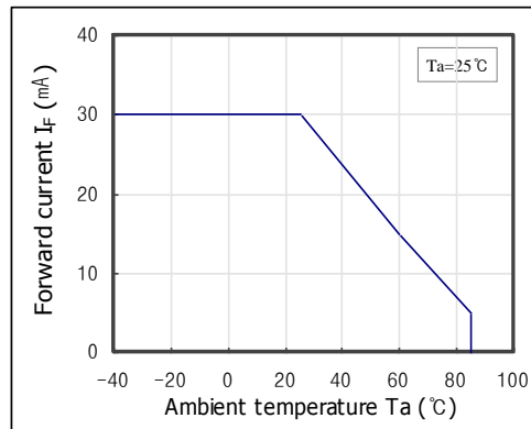
Forward Current Dissipation Curve
