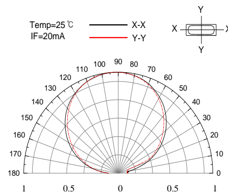
Radiation Angle
