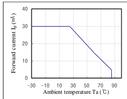
Forward Current Dissipation Curve
