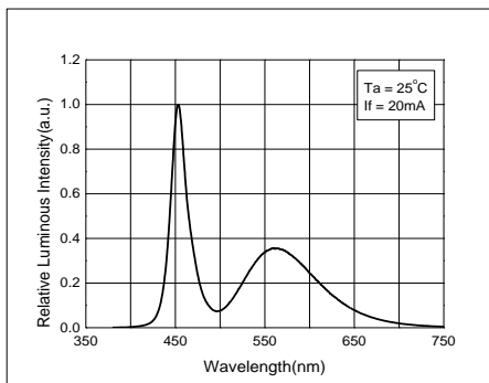
Relative Spectral Emission
