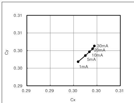
Forward Current vs Chromaticity Diagram
