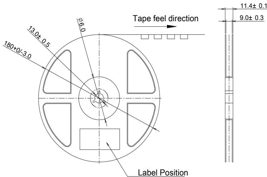
< 7" Reel >
