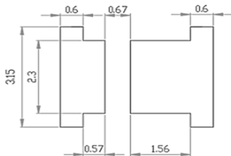
[Recommended PCB Solder Pad]
