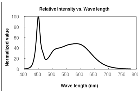
CCT : 5000 K (80 CRI)
