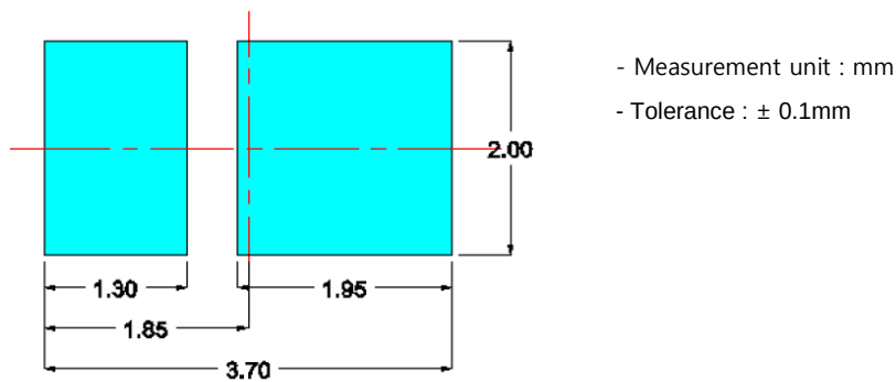
[Recommended PCB Solder Pad]
