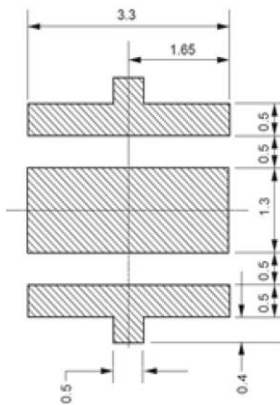
[Recommended PCB Solder Pad]
