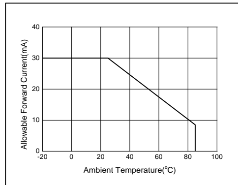
Forward Current Dissipation Curve
