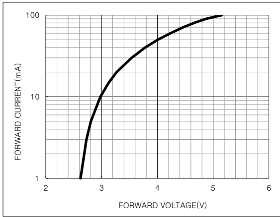
Forward Current vs Forward Voltage (Per die)
