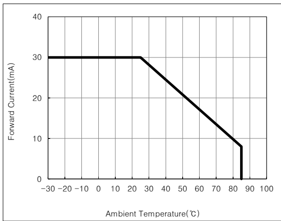
Forward Current vs. Ambient Temperature (Per die)
