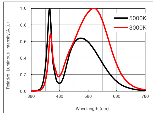
Relative Spectral Emission (Per die)
