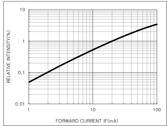
Relative Luminous Intensity vs Forward Current (Per die)
