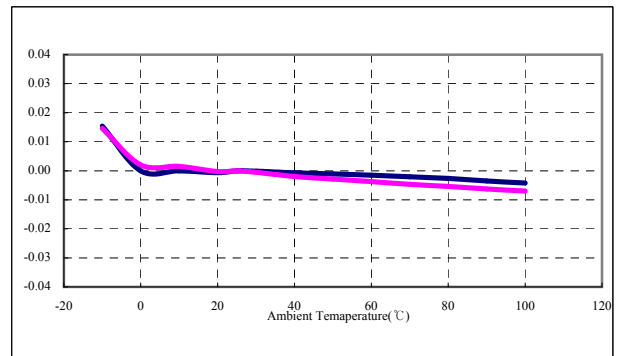
Relative Chromaticity vs Ambient Temperature (Warm White)
