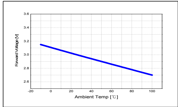
Ambient Temperature vs Forward Voltage
